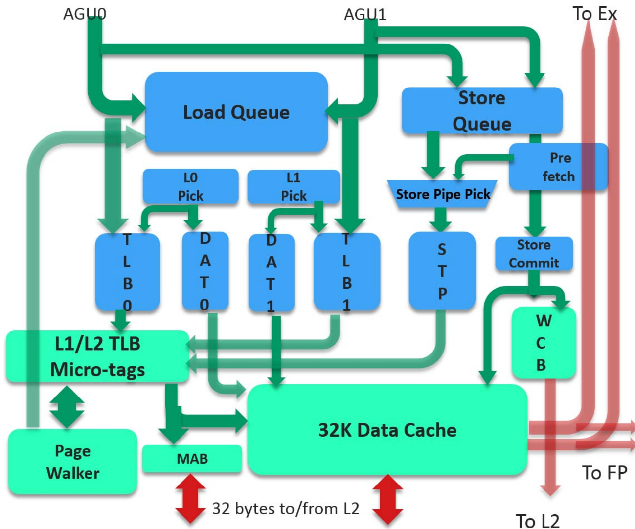
Figure 7. Load-Store Unit
